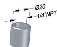
VENT BOSS
